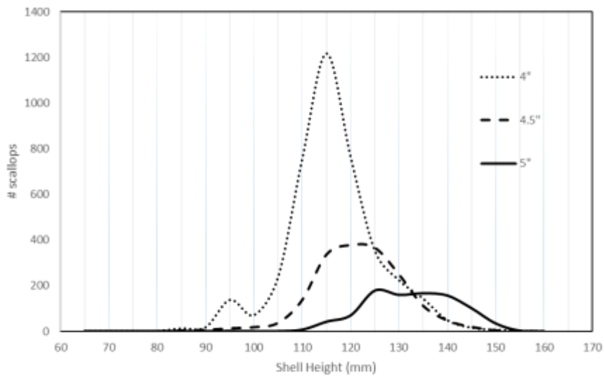
Figure 5. Number and size of sea scallops caught in dredges with 4", 4.5", and 5" rings.
