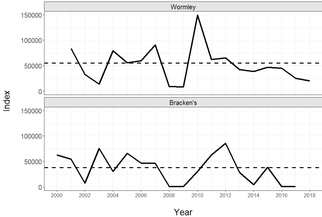
Figure 2. Abundance indices and time series average calculated by the area-under-the-curve method for glass American Eels from Wormley Pond (York River estuary). Time series averages are shown as dotted lines. Sampling at Bracken's Pond ended in 2017.
