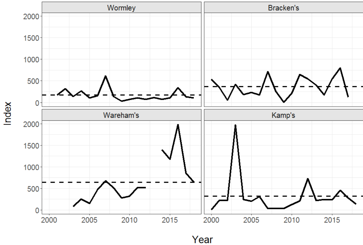
Figure 6. Abundance indices and time series average calculated by the area-under-the-curve method for elver American Eels from Wormley Pond, Bracken's Pond (York River estuary), Wareham's Pond (James River estuary) and Kamp's Millpond (Rappahannock River estuary). Time series averages are shown as dotted lines. Sampling at Bracken's Pond ended in 2017.
