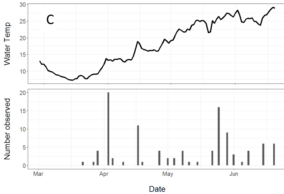
Figure 7 continued. Water temperature (top panel) and elver American Eel catches (bottom panel) from (C) Kamp's Millpond in 2018. Note axis scales are not uniform.
