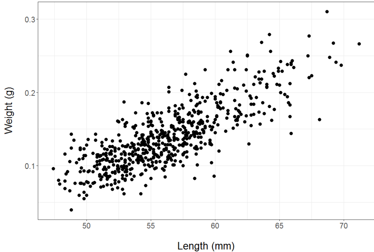
Figure 8. Length-weight relationship for glass American Eels from the York River estuary, 2018. Average TL = 56.3 mm, average weight = 0.140 g, N = 612 eels.
