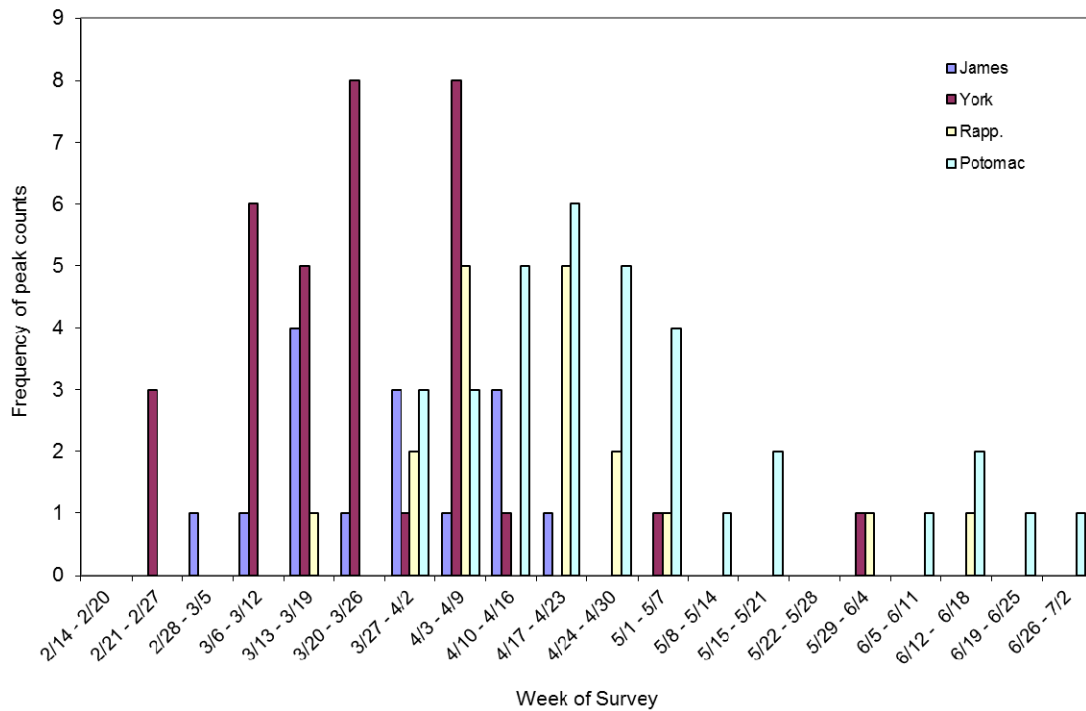
Figure 5. Survey week during which peak counts of glass eels were observed at each site from 2001 to 2018. Two sites are monitored in the York and Potomac estuaries each year ( n = 34 observations per river; only one site was monitored in each river after 2017). In the James River estuary, one site was monitored continuously since 2003, though this site was not accessible in 2013 ( n = 15 observations). In the Rappahannock River estuary, one site was monitored each year ( n = 18 observations). Potomac River data are from Tuckey and Fabrizio (2018).
