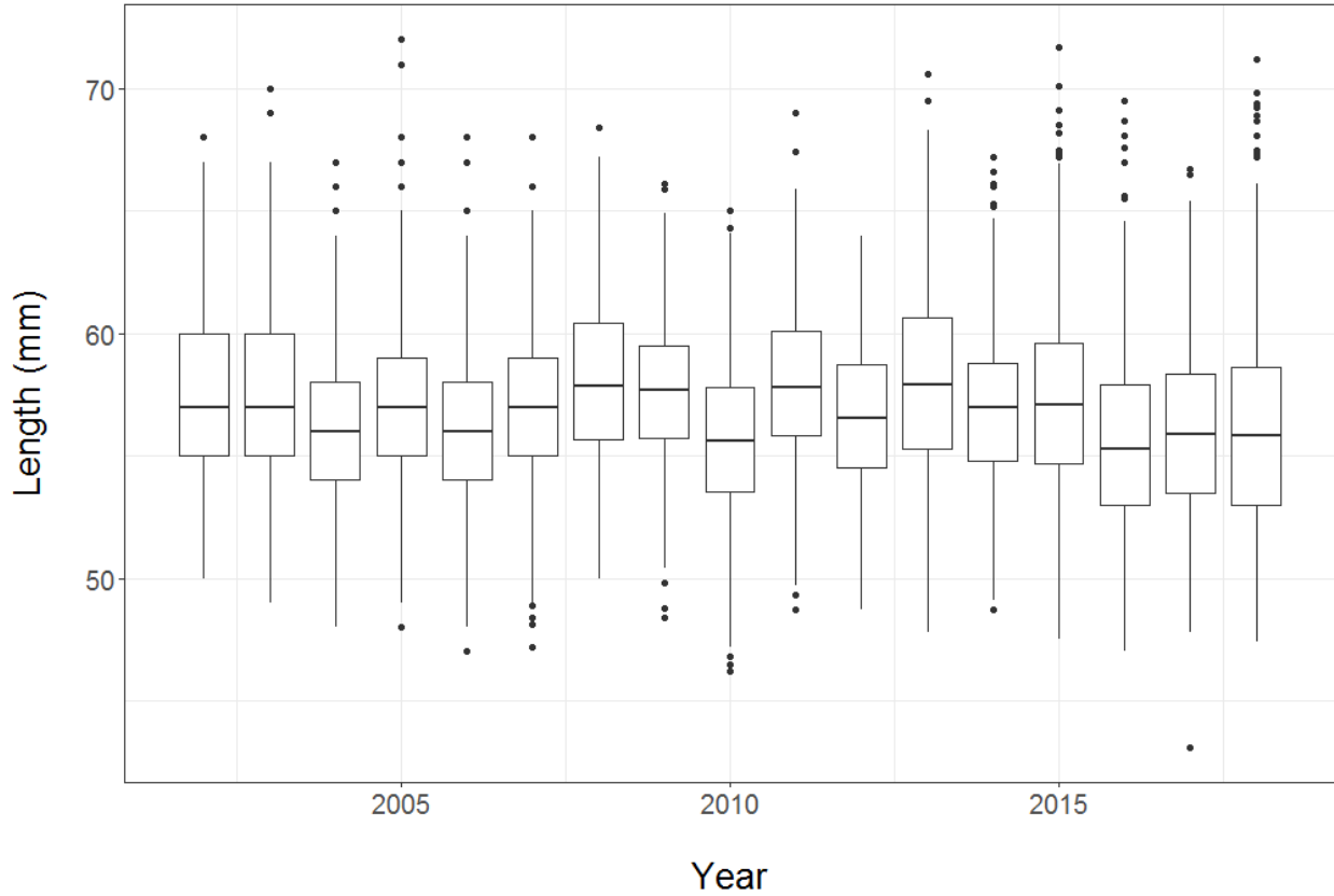
Figure 9. Total length (mm) of glass American Eels collected with Irish Eel ramps from 2002 to 2018 from Wormley Pond in the York River estuary, Virginia. Long-term mean 56.8 mm ( n = 18 years). The thick line in the center of the box indicates the median, the boxes indicate the 25 th and 75 th percentiles, the vertical lines indicate the 5 th and 95 th percentiles, and the dots indicate more extreme observations.
