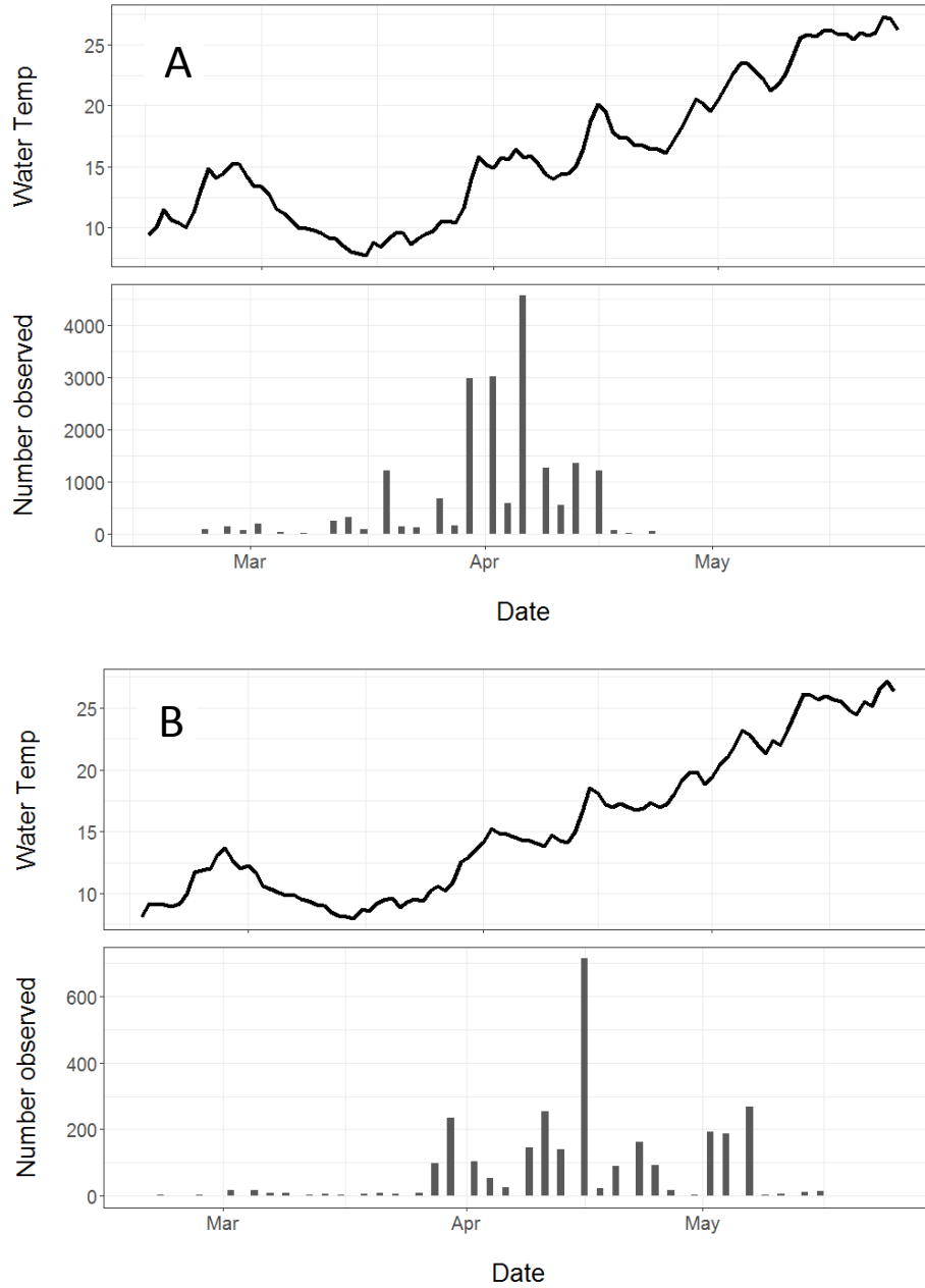
Figure 4. Water temperature (top panel) and glass American Eel catches (bottom panel) from (A) Wormley Pond, and (B) Wareham's Pond in 2018. Note axis scales are not uniform.
