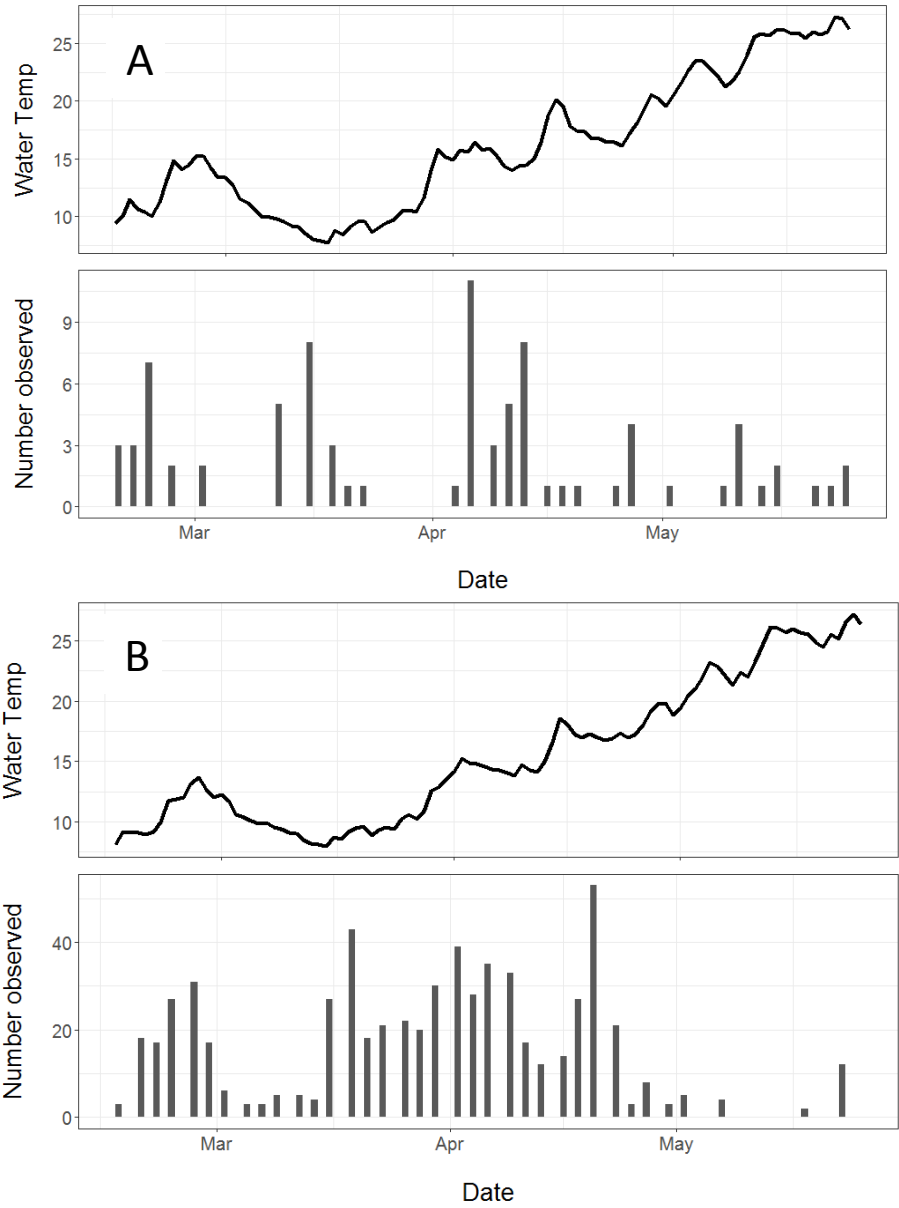
Figure 7. Water temperature (top panel) and elver American Eel catches (bottom panel) from (A) Wormley Pond, and (B) Wareham's Pond in 2018. Note axis scales are not uniform.
