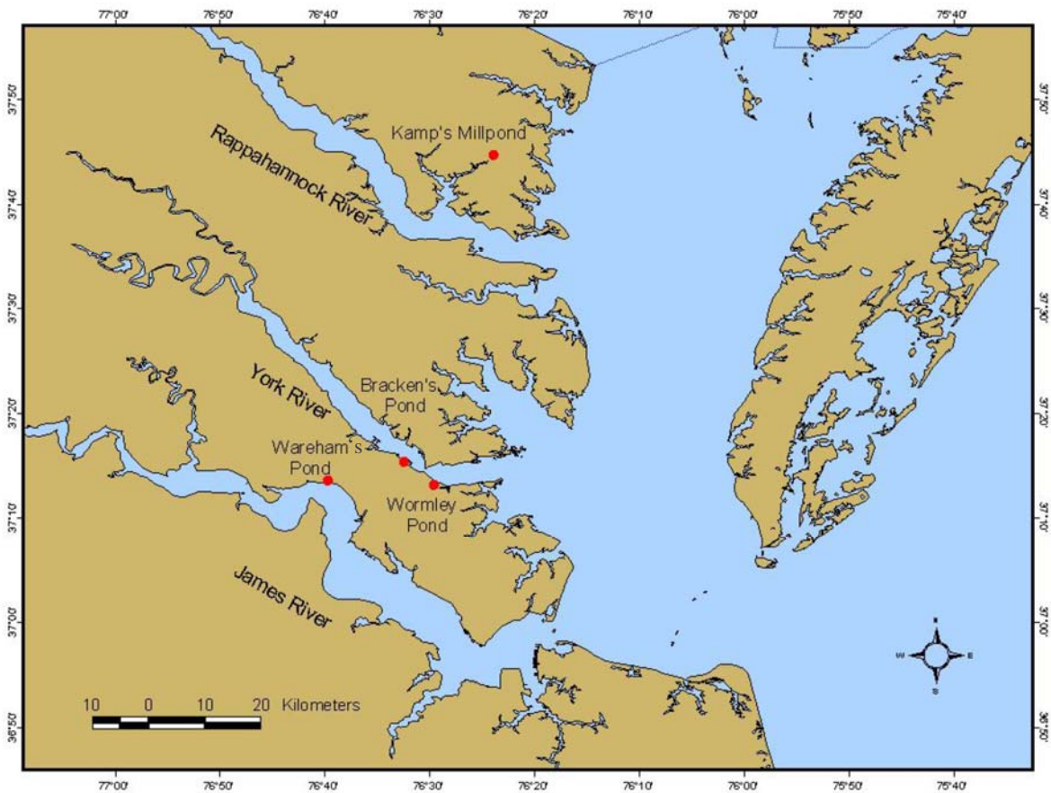
Figure 1. American Eel sampling sites in sub-estuaries of the Chesapeake Bay: the Rappahannock (Kamp's Millpond), York (Wormley Pond), and James (Wareham's Pond) estuaries, Virginia, 2018. Sampling at Bracken's Pond ended in 2017.
