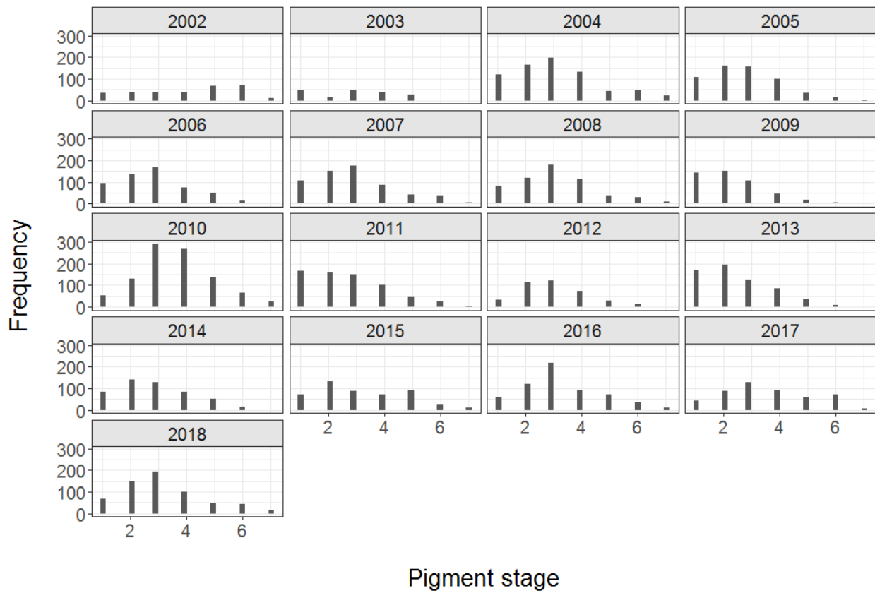
Figure 10. Frequency of pigment stages for glass eels by year for the York River estuary.
