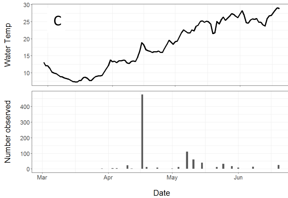
Figure 4 continued. Water temperature (top panel) and glass American Eel catches (bottom panel) from (C) Kamp's Millpond in 2018. Note axis scales are not uniform.
