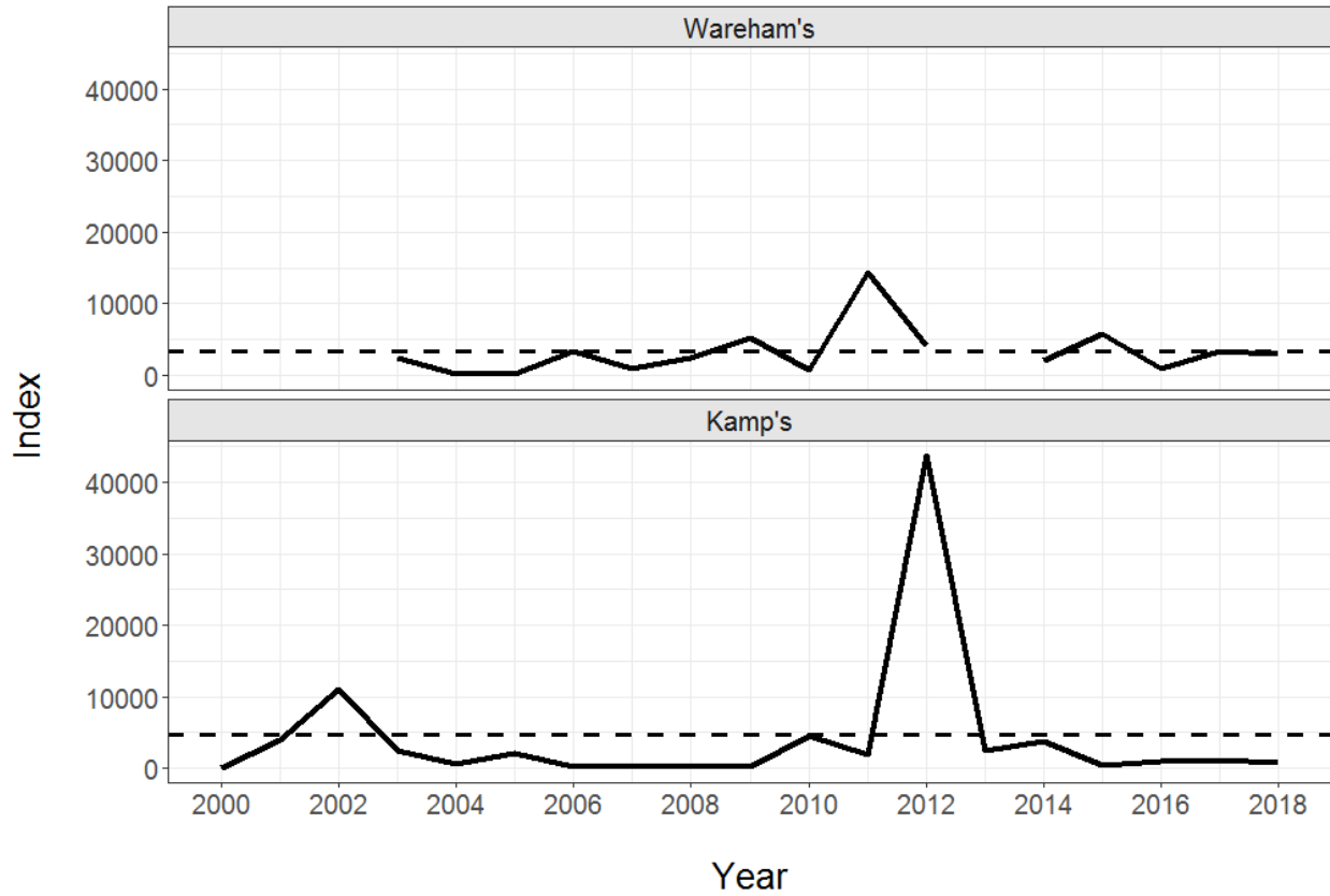
Figure 3. Abundance indices and time series average calculated by the area-under-the-curve method for glass American Eels from Wareham's Pond (James River estuary) and Kamp's Millpond (Rappahannock River estuary). Time series averages are shown as dotted lines. Wareham's Pond was not sampled in 2013 due to dam construction at our sampling site.
