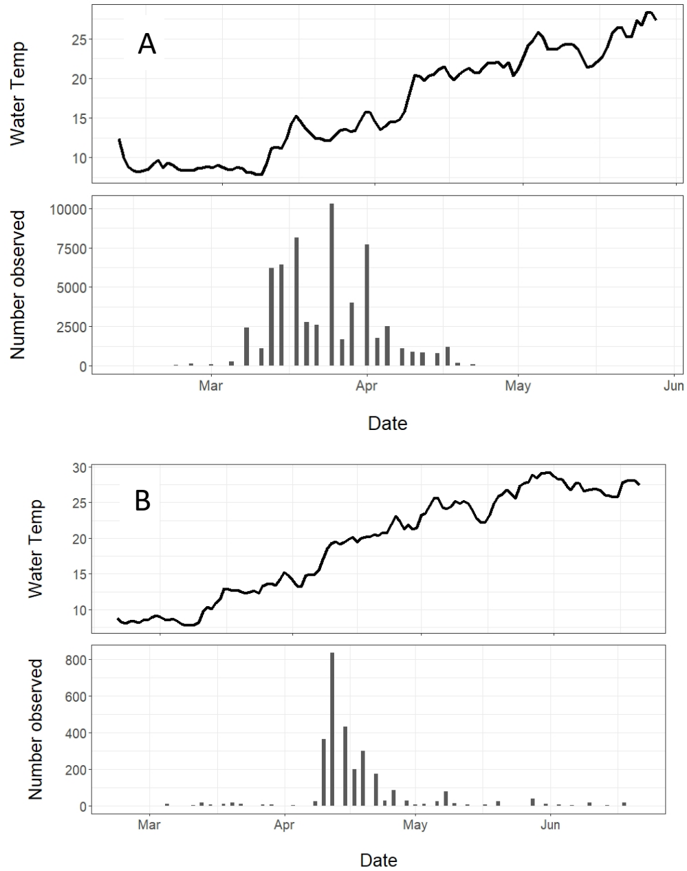
Figure 4. Water temperature (top panel) and glass American Eel catches (bottom panel) from (A) Wormley Pond, and (B) Wareham's Pond in 2019. Note axis scales are not uniform.
