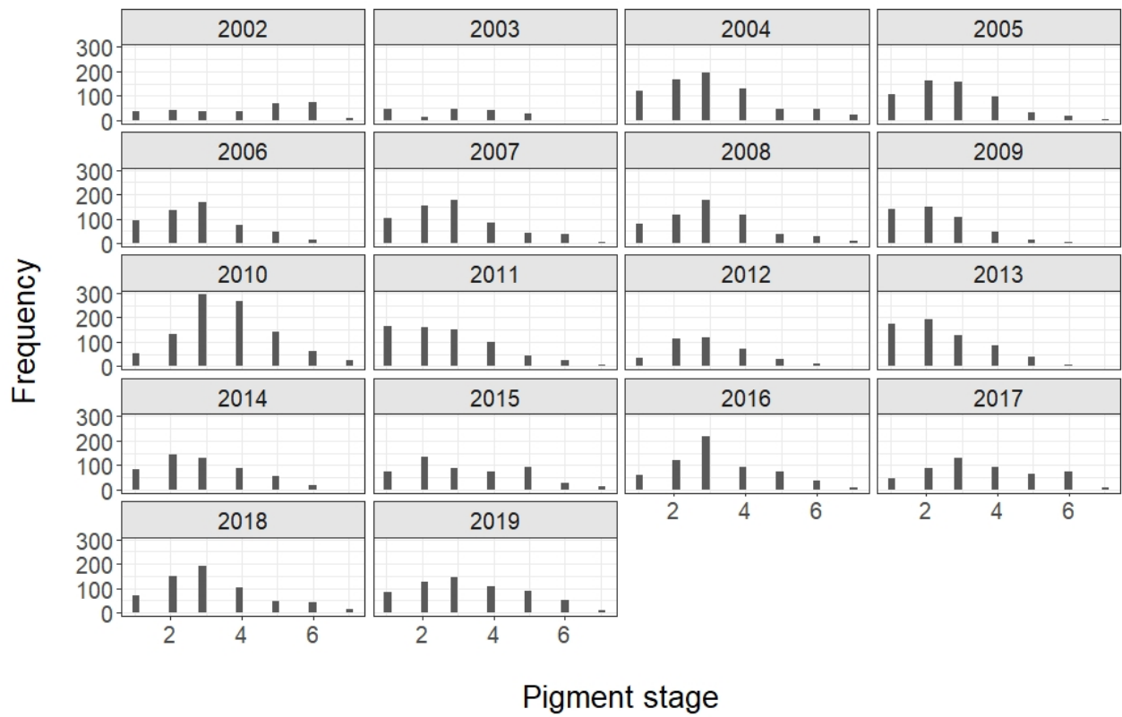
Figure 10. Frequency of pigment stages for glass eels by year for the York River estuary.
