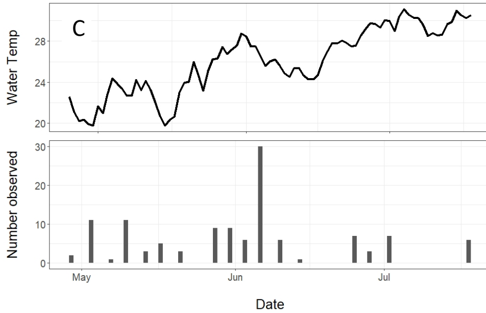
Figure 4 continued. Water temperature (top panel) and glass American Eel catches (bottom panel) from (C) Kamp's Millpond in 2019. Note axis scales are not uniform.
