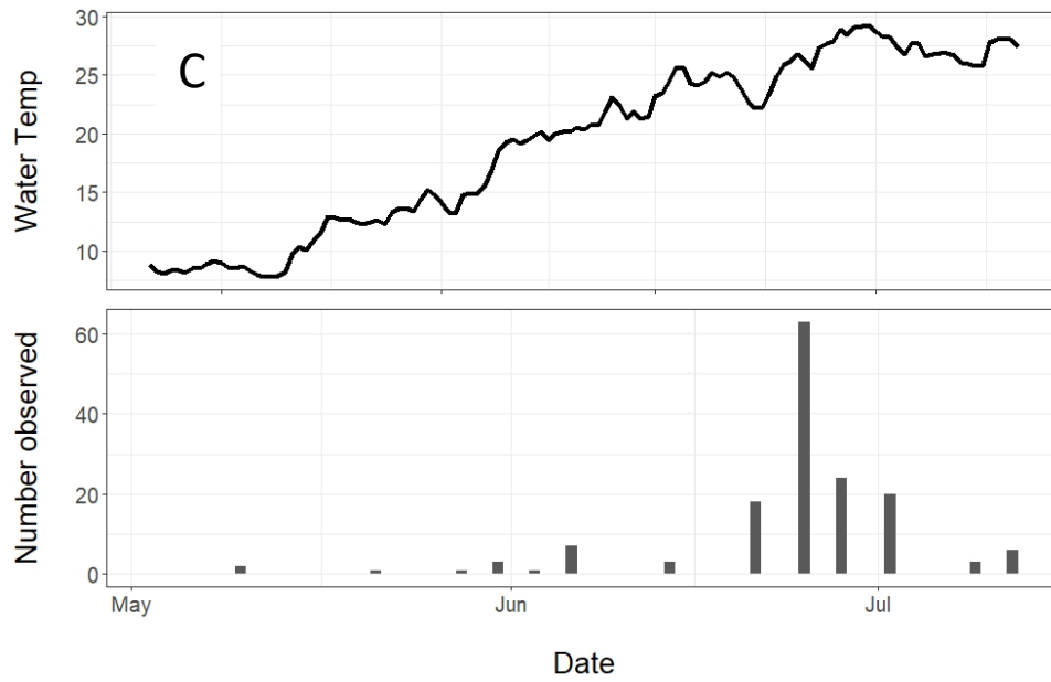
Figure 7 continued. Water temperature (top panel) and elver American Eel catches (bottom panel) from (C) Kamp's Millpond in 2019. Note axis scales are not uniform.
