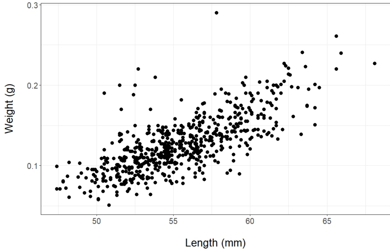
Figure 8. Length-weight relationship for glass American Eels from the York River estuary, 2019. Average TL = 55.5 mm, average weight = 0.127 g, N = 615 eels.
