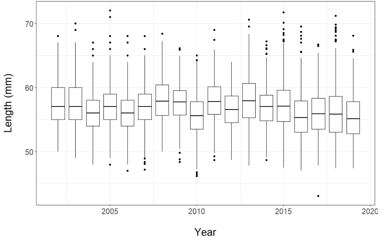
Figure 9. Total length (mm) of glass American Eels collected with Irish Eel ramps from 2002 to 2019 from Wormley Pond in the York River estuary, Virginia. Long-term mean 56.8 mm (n = 18 years). The thick line in the center of the box indicates the median, the boxes indicate the 25 th and 75 th percentiles, the vertical lines indicate the 5 th and 95 th percentiles, and the dots indicate more extreme observations.
