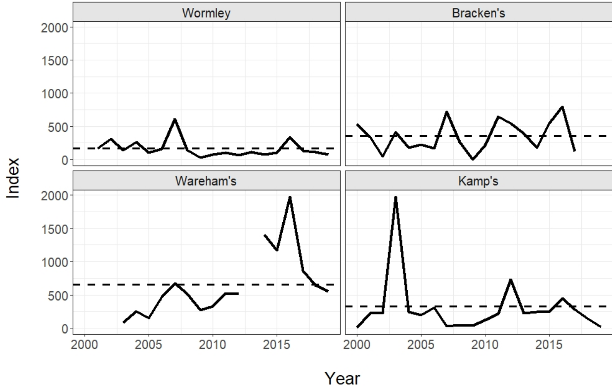
Figure 6. Abundance indices and time series average calculated by the area-under-the-curve method for elver American Eels from Wormley Pond, Bracken's Pond (York River estuary), Wareham's Pond (James River estuary) and Kamp's Millpond (Rappahannock River estuary). Time series averages are shown as dotted lines. Wareham's Pond was not sampled in 2013 due to spillway construction at our sampling site and sampling at Bracken's Pond ended in 2017.
