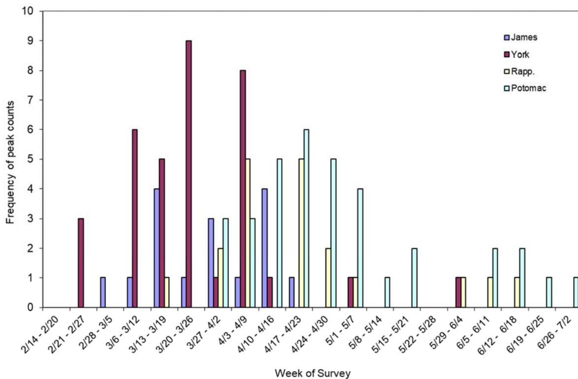
Figure 5. Survey week during which peak counts of glass eels were observed at each site from 2001 to 2019. Two sites were monitored in the York and Potomac estuaries each year from 2001 to 2017, and one site thereafter (n = 35 observations per river). In the James River estuary, one site was monitored continuously since 2003, though this site was not accessible in 2013 (n = 16 observations). In the Rappahannock River estuary, one site was monitored each year (n = 19 observations). Potomac River data are from Tuckey and Fabrizio (2019).
