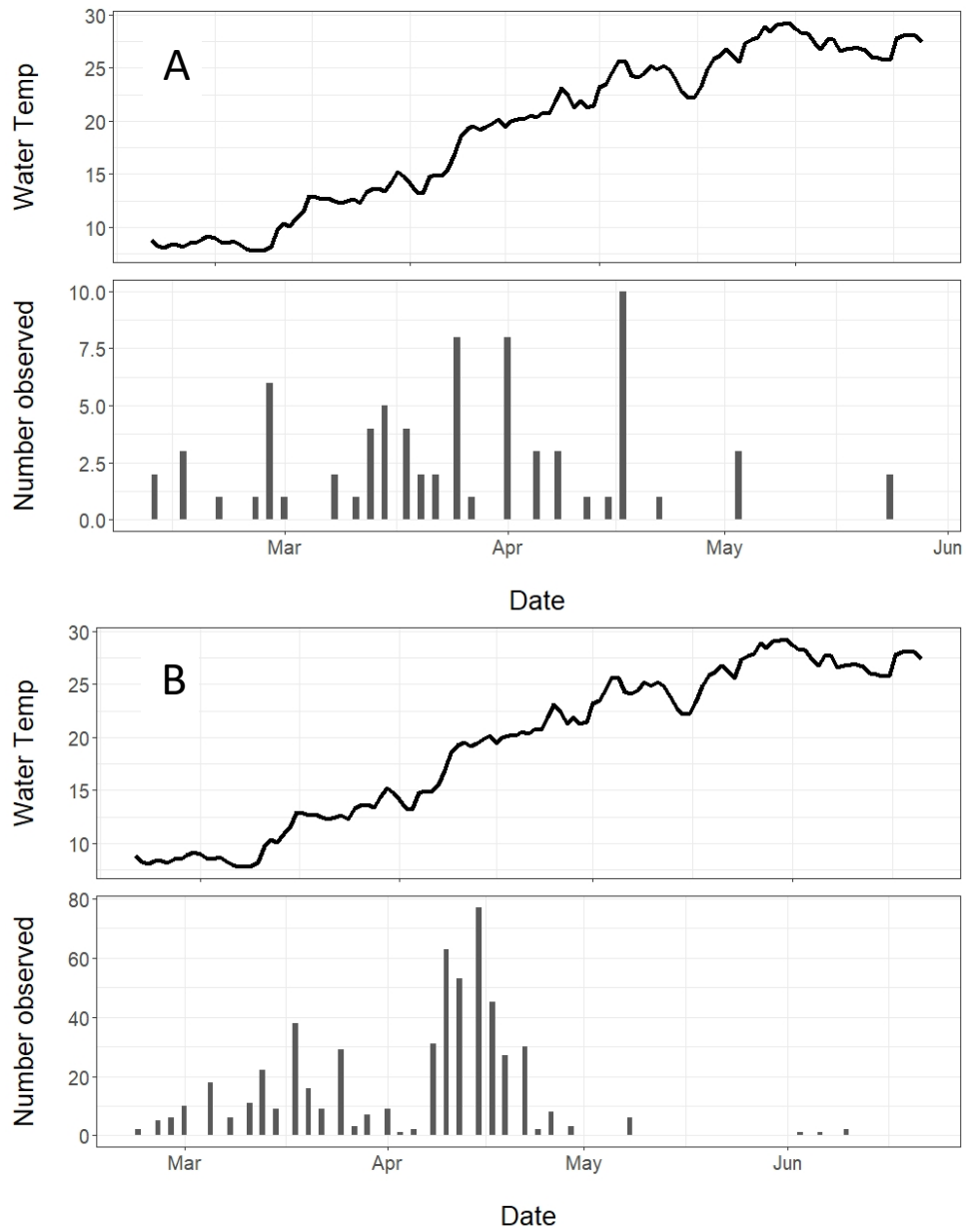
Figure 7. Water temperature (top panel) and elver American Eel catches (bottom panel) from (A) Wormley Pond, and (B) Wareham's Pond in 2019. Note axis scales are not uniform.
