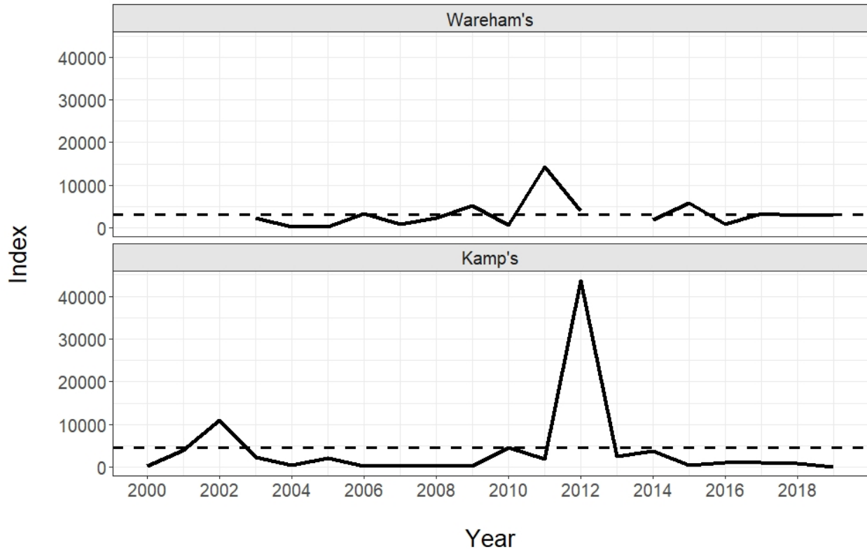
Figure 3. Abundance indices and time series average calculated by the area-under-the-curve method for glass American Eels from Wareham's Pond (James River estuary) and Kamp's Millpond (Rappahannock River estuary). Time series averages are shown as dotted lines. Wareham's Pond was not sampled in 2013 due to spillway construction at our sampling site.
